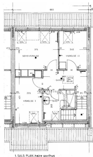
1½ Plan – 110 m 2
