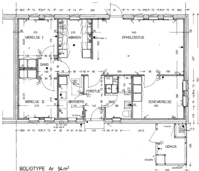
1 Plan – 94 m 2
