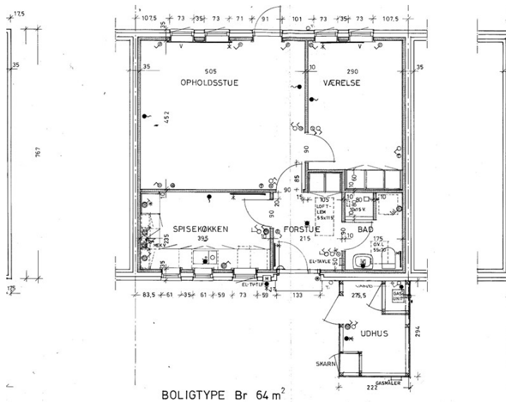
1 Plan – 64 m 2
