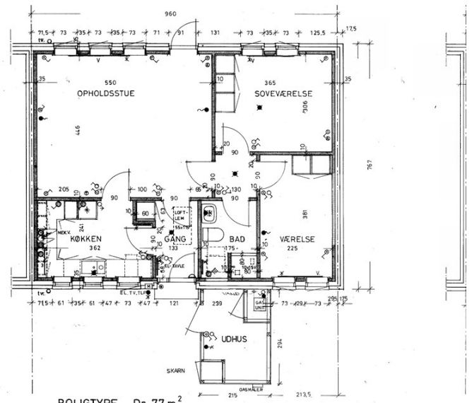
1 Plan – 77 m 2
